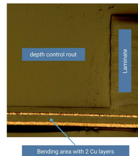
cross-section view
